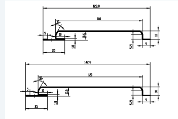
CROSS-SECTION PROFILE
