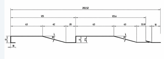
CROSS-SECTION PROFILE
